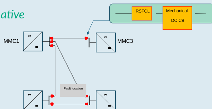
RSFCL in a multi-terminal electrical diagram
