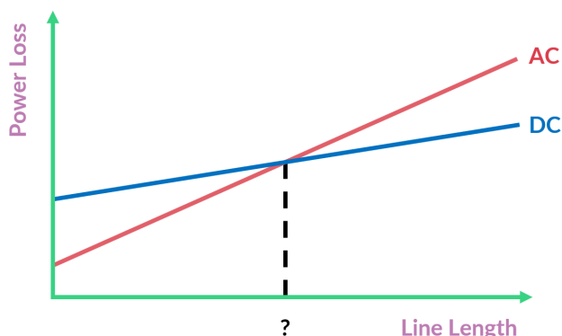
Publication EPE 2021: Break-even distance for MVDC electricity networks according to power loss criteria
